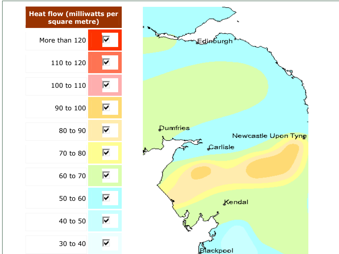
Figure 5-5: Heat flow per square metre of Northern England and Southern Scotland
