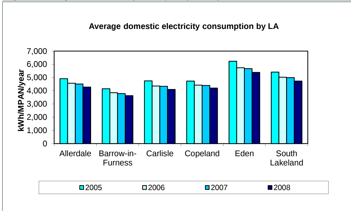
Figure 3-4: Average domestic electricity consumption by authority
