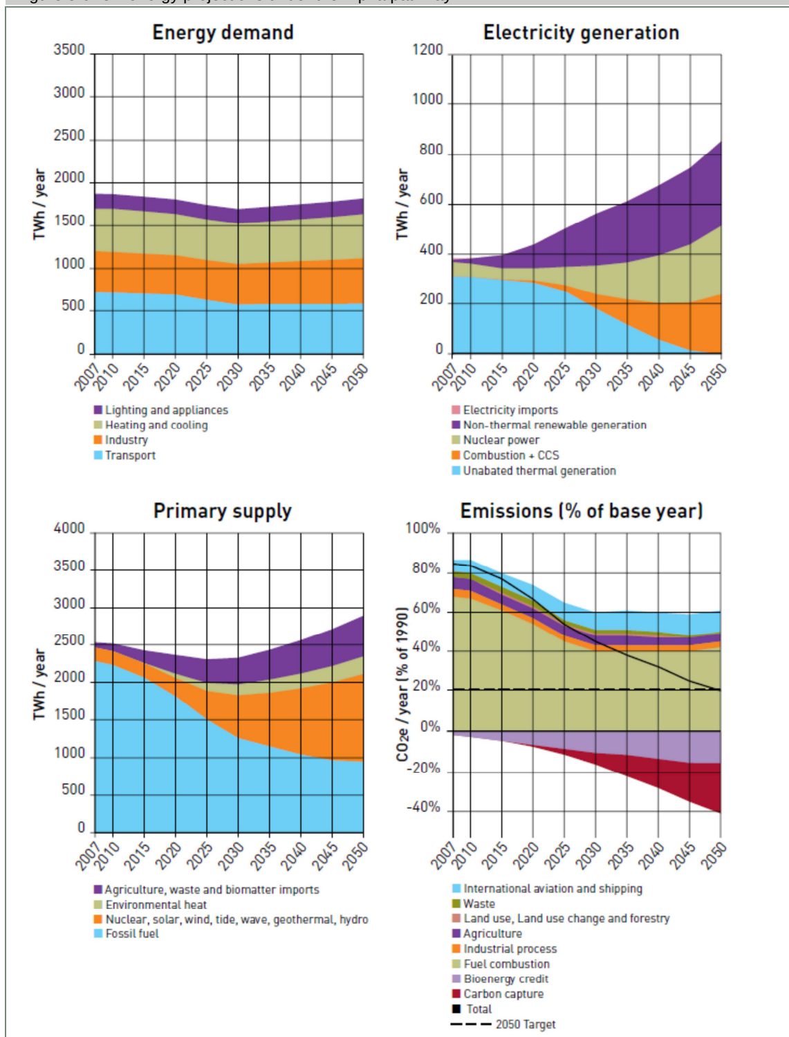
Figure 3-9: UK energy projections under the Alpha pathway
