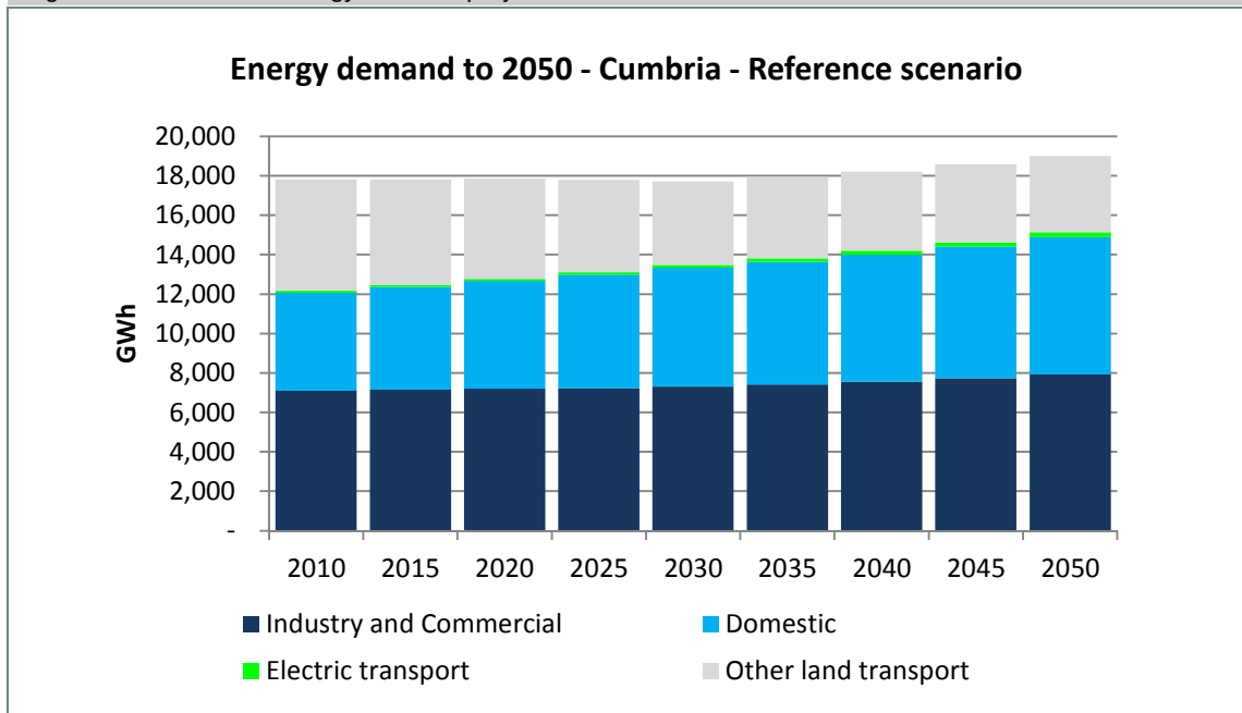
Figure 3-10: Cumbria energy demand projections under the Reference case
