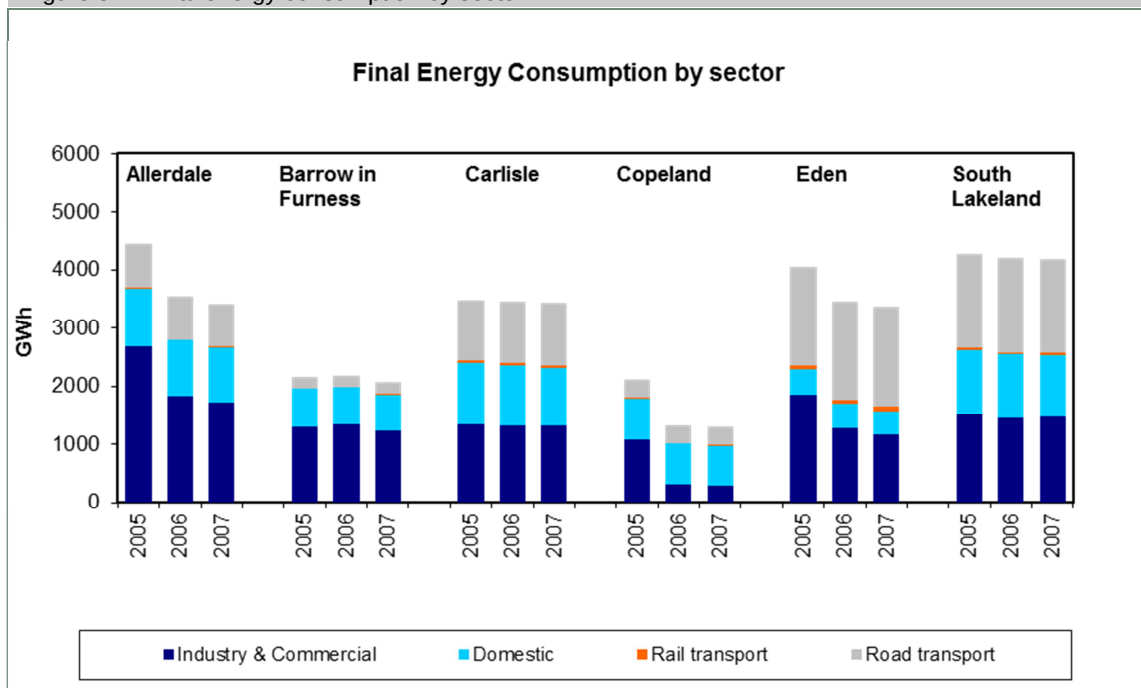
Figure 3-1: Final energy consumption by sector
