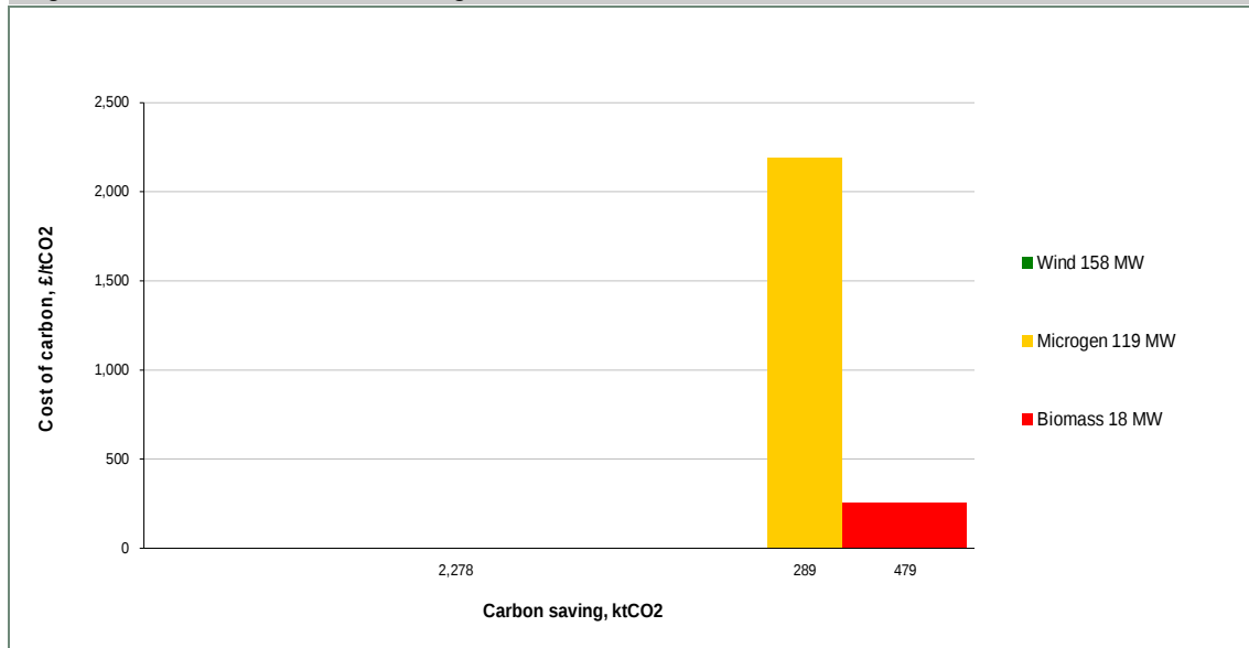
Figure 7-1: Total cost v carbon savings
